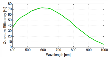
MV-CA032-10GM 量子效率
